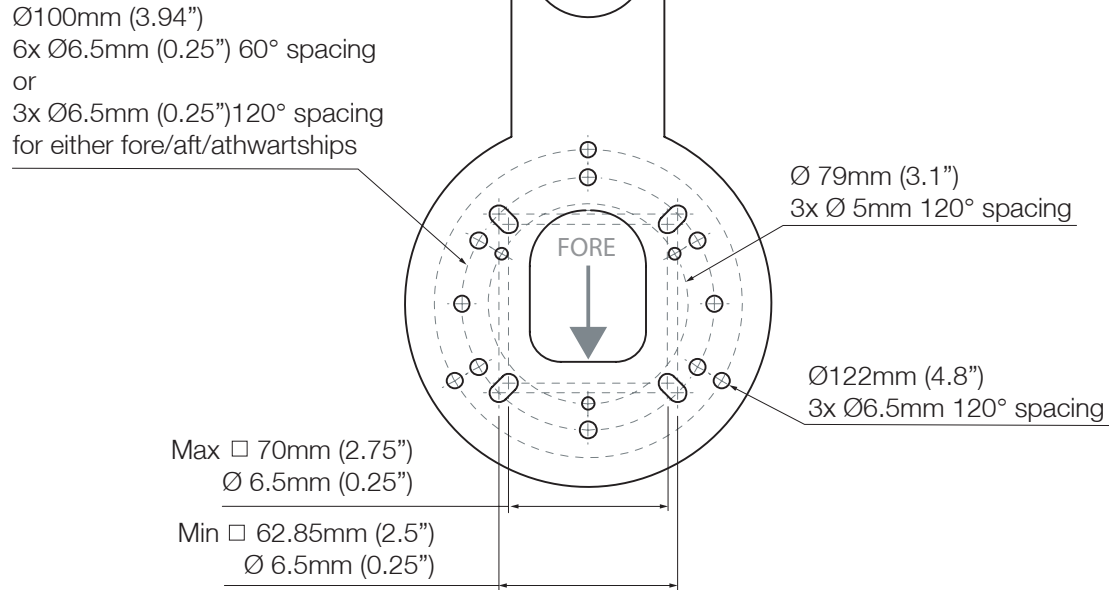
Camera Mounting plate
