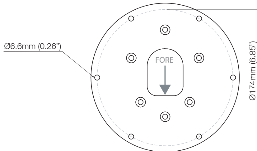
Flir M100/200 series camera plate
